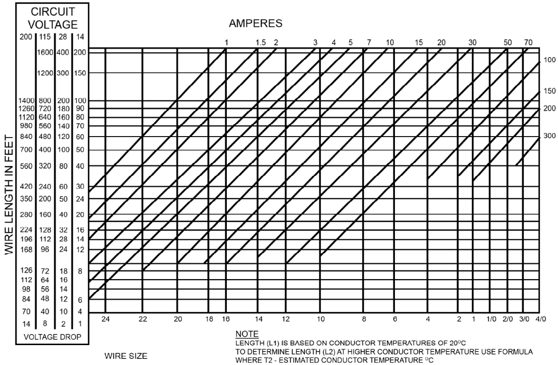
WIRE SIZE VOLTAGE DROP CHART INTERMITTENT FLOW AT 20° TIN-PLATED MIL-W-27759 CONDUCTOR
