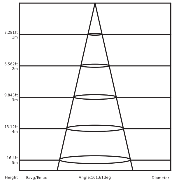
Illuminance Characteristics
